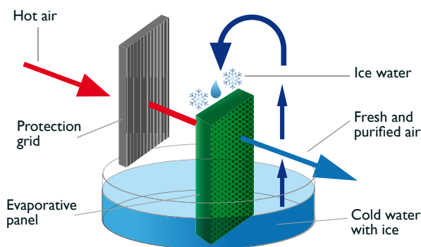
2 Ice boxes to increase the cooling effect
